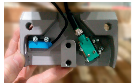
Integrated cable routing in the fork for energy supply and data transmission
